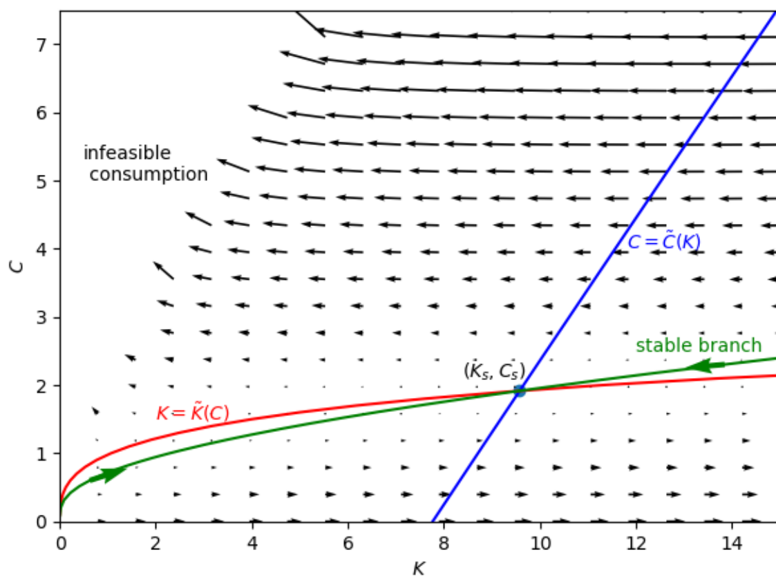
Fig. 34.1: Stable Manifold and Phase Plane
